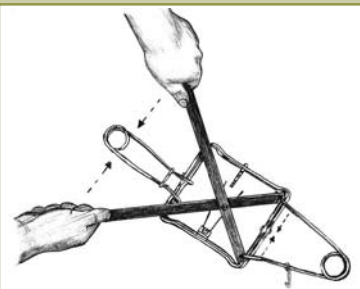
Figure SK3a. Using setting tool
